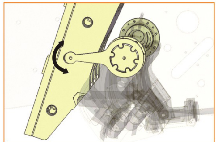
可調整破碎行程的偏心結構 Adjustable stroke eccentric sleeve mechanism
