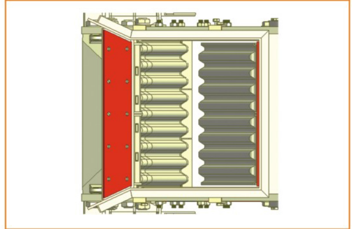
合適之破碎腔口配合入料槽 Suitable crusher cavity with feed chute
